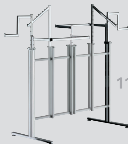
4168 Komet stand 2 x 600 mm axis Equipped with: 2 Conf. Frame 4560 2 Tiereds 4224, 450 mm 2 Tiered arms 4243, 350 mm
